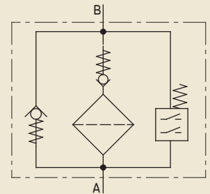
Hydraulic plan 2
