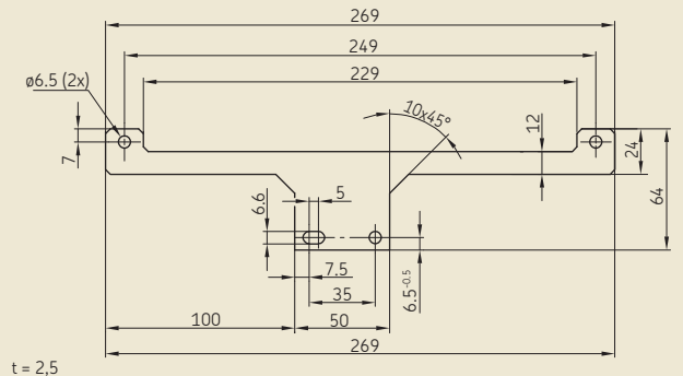
Filter plate 881-290-270
