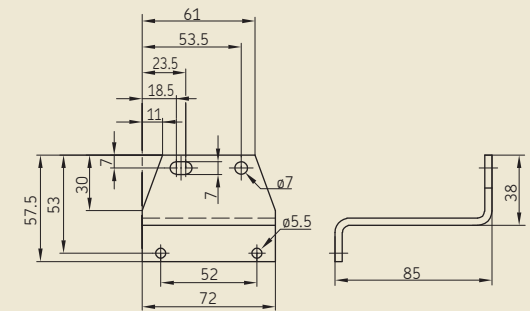
Mounting bracket 881-280-050
